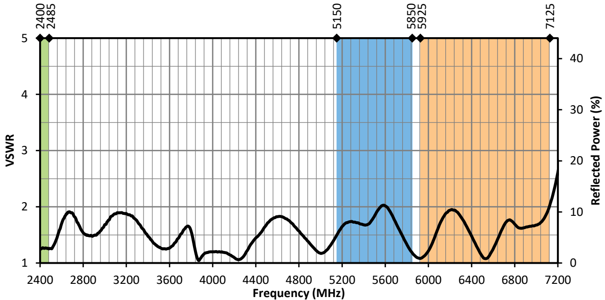
Figure 4. ANT-W63WS5-ccc VSWR, Straight
